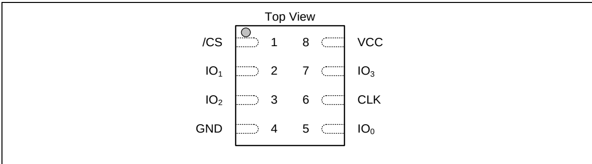
Figure 1b. W74M12FV Pad Assignments, 8-pad WSON 6x5-mm (Package Code ZP)
