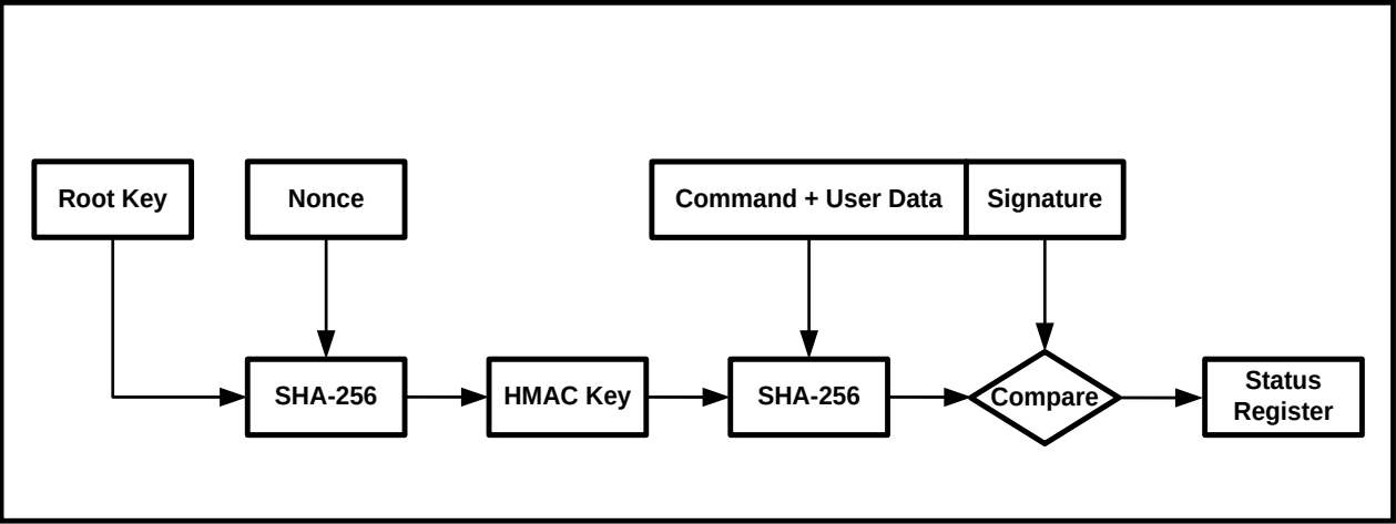
Figure 2. W74M12FV Operation Diagram
