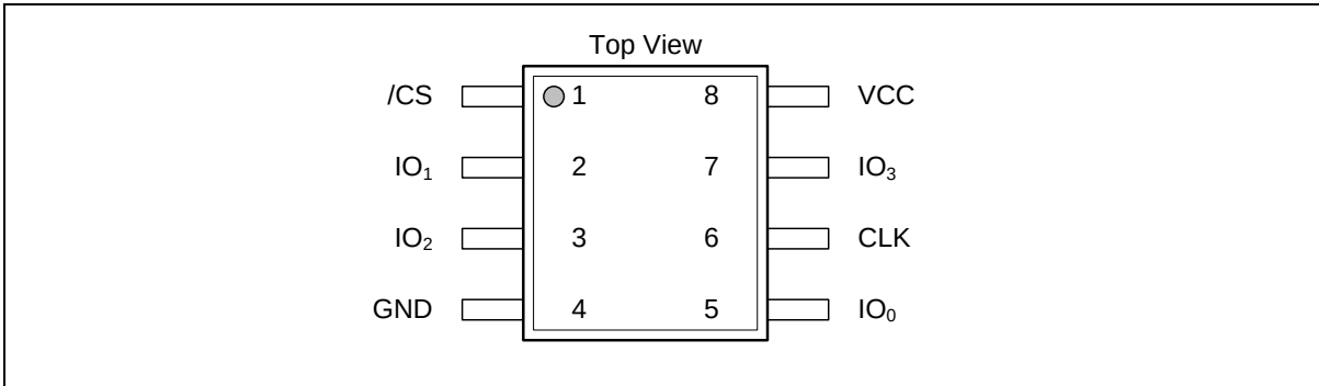
Figure 1a. W74M12FV Pin Assignments, 8-pin SOIC 208-mil (Package Code SS)
